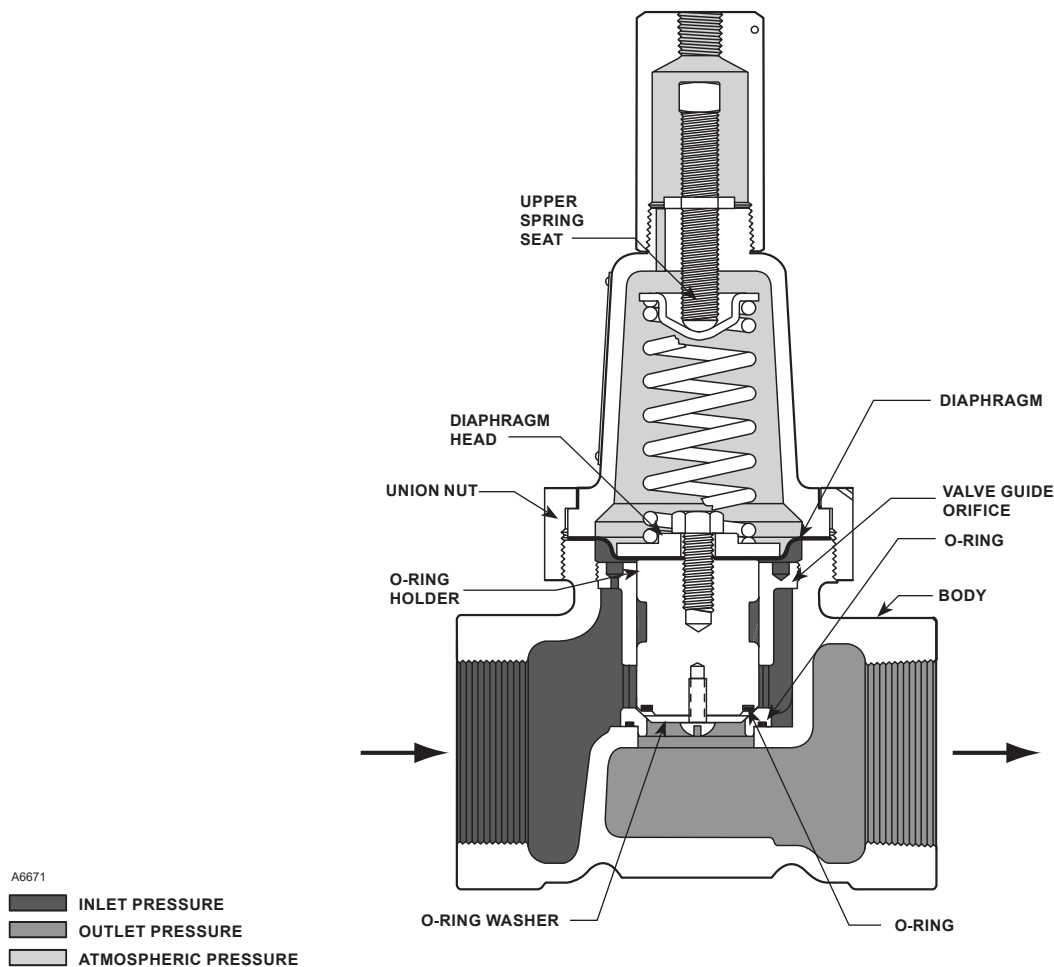
Figure 2. 1805 Series Operational Schematic
