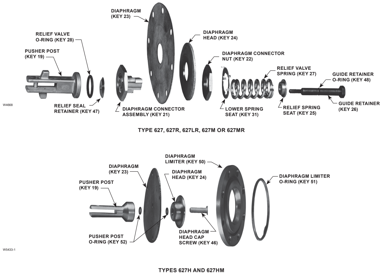
Figure 6. Diaphragm Assemblies
