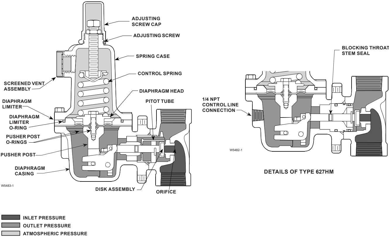
Figure 7. Types 627H and 627HM Operational Schematics
