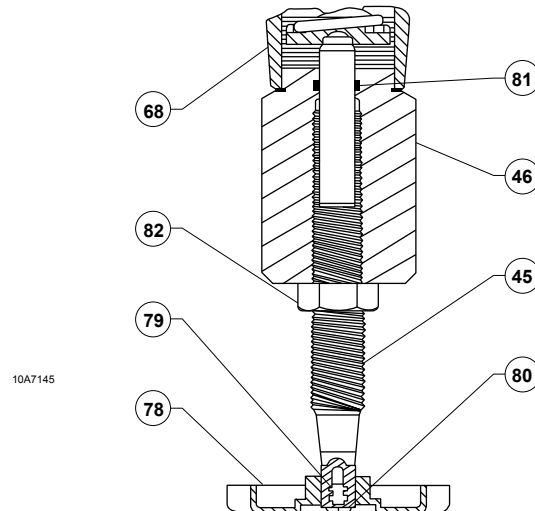
Figure 8. O-ring Sealed Handwheel
