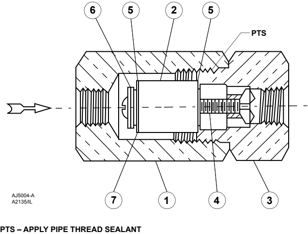
Figure 16. Standard P590 Series Filter Assembly
