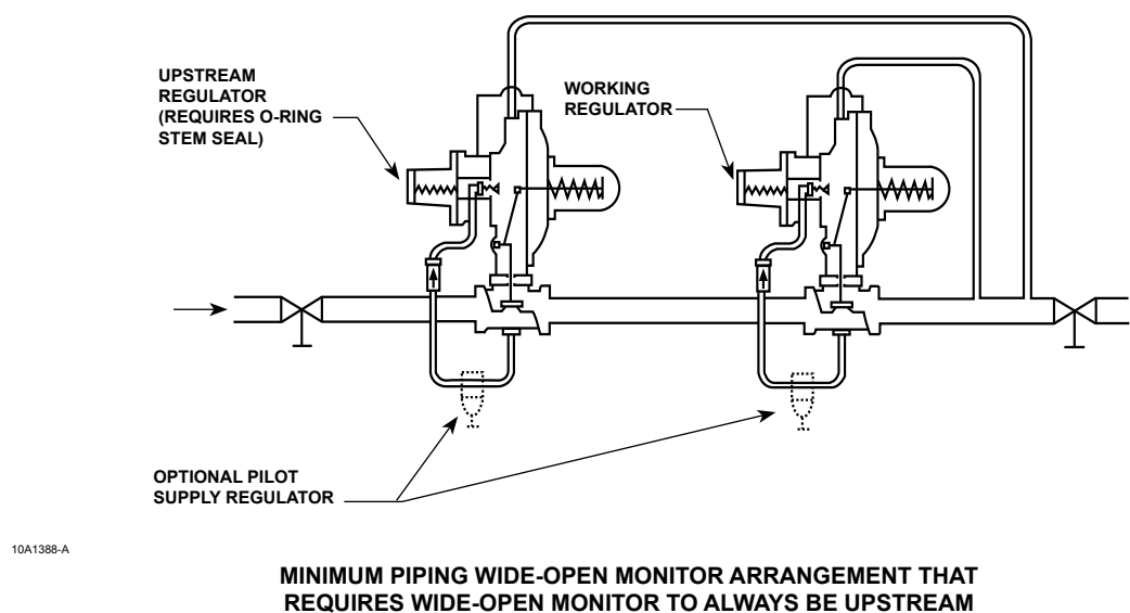
Figure 11. Typical Wide-Open Monitor Installations
