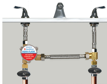
Flash Valve Installed
