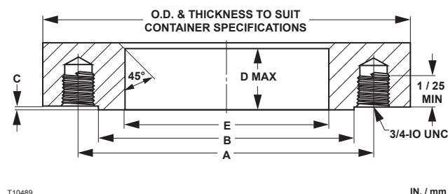
Figure 2. Tank Flange Dimensions
