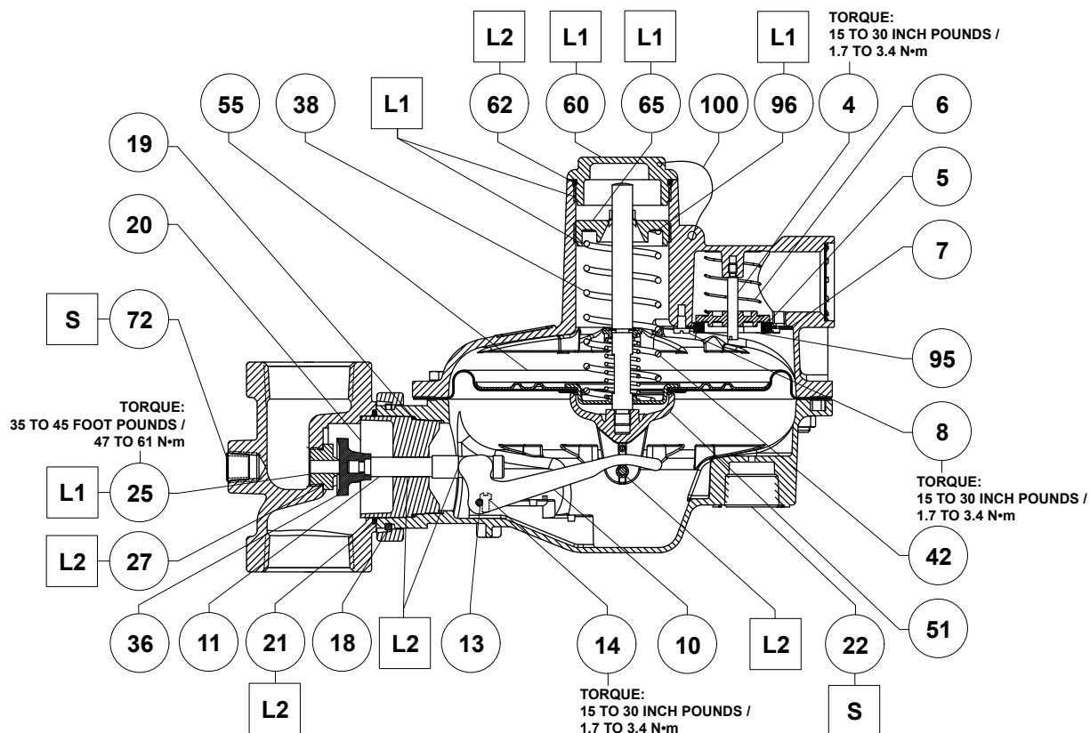
MAIN VALVE
