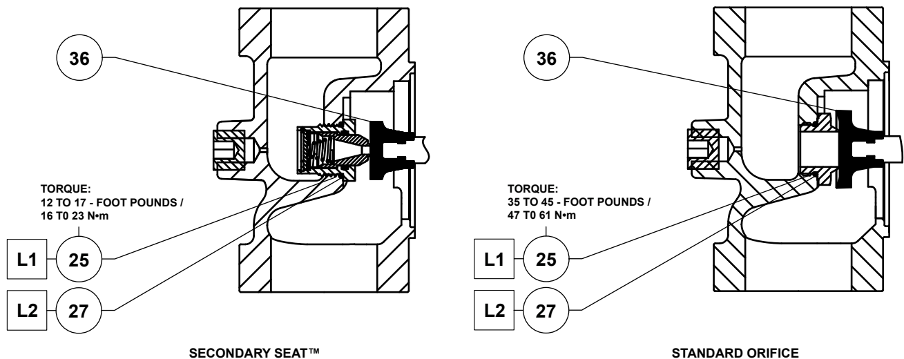
Figure 6. CS200 Series Diaphragm Assemblies
