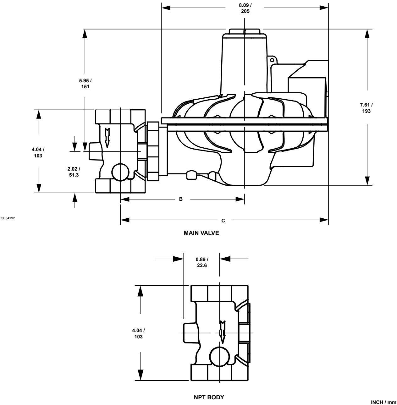
Figure 10. Dimensions
