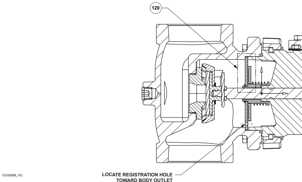
Figure 13. CS800 Series with Stabilizer Cartridge Assembly
