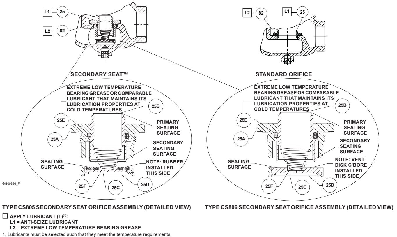
Figure 19. CS800 Series Base Orifice and Secondary Seat (For Types CS805 and CS806) Assemblies (continued)
