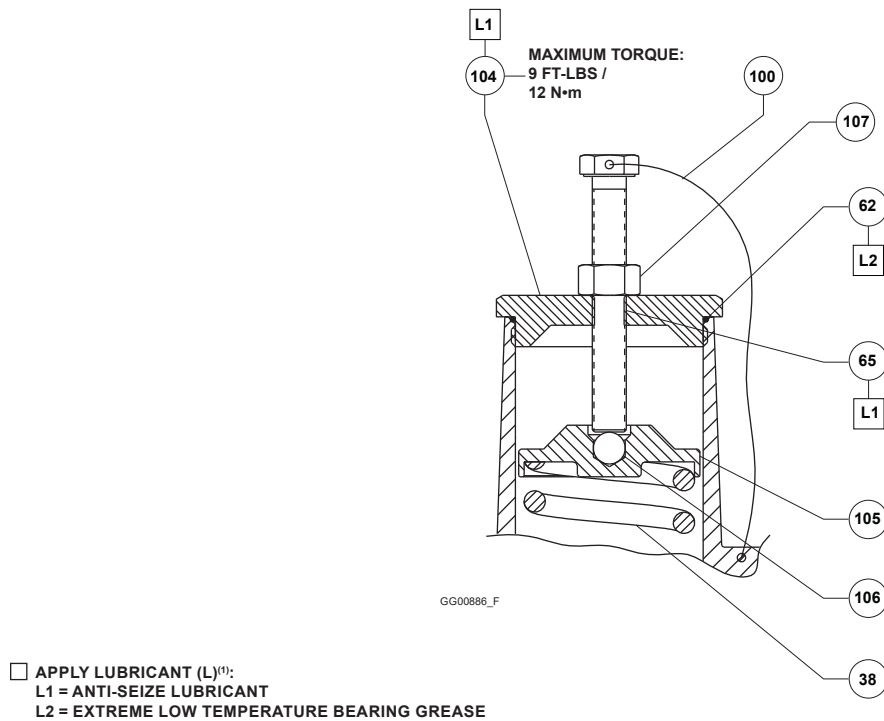
Figure 16. CS800 Series Control Spring Adjustment Assemblies (continued)
