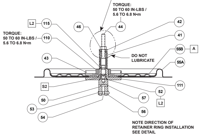
TYPE CS800/CS820 TOKEN RELIEF LOW FLOW
