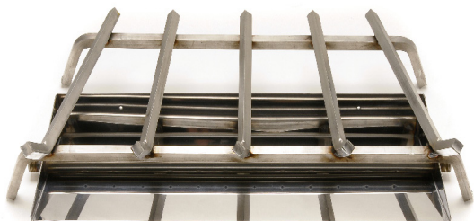
Figure 4.2 Center Stainless Grate Over Stainless Burner Pan
