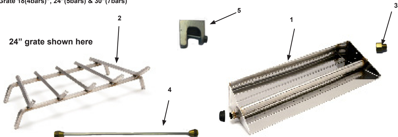
Exploded Parts Diagram
