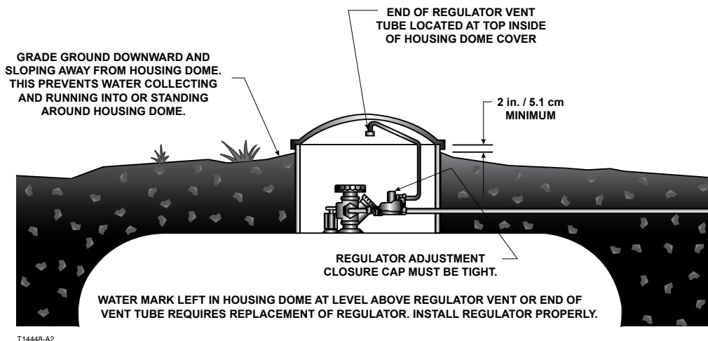
Figure 5. Underground Installation
