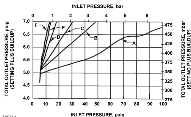
5 psig / 0.34 bar TYPE S202H REGULATOR WITH SEAT BLOCKED OPEN BY ONE 1/8-INCH / 3.2 mm DIAMETER WIRE
