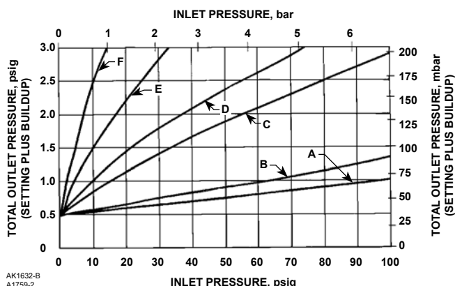
7 INCHES W.C. / 17 mbar TYPE S202 OR S206 REGULATOR WITH SEAT BLOCKED OPEN BY TWO 1/8-INCH / 3.2 mm DIAMETER WIRES
